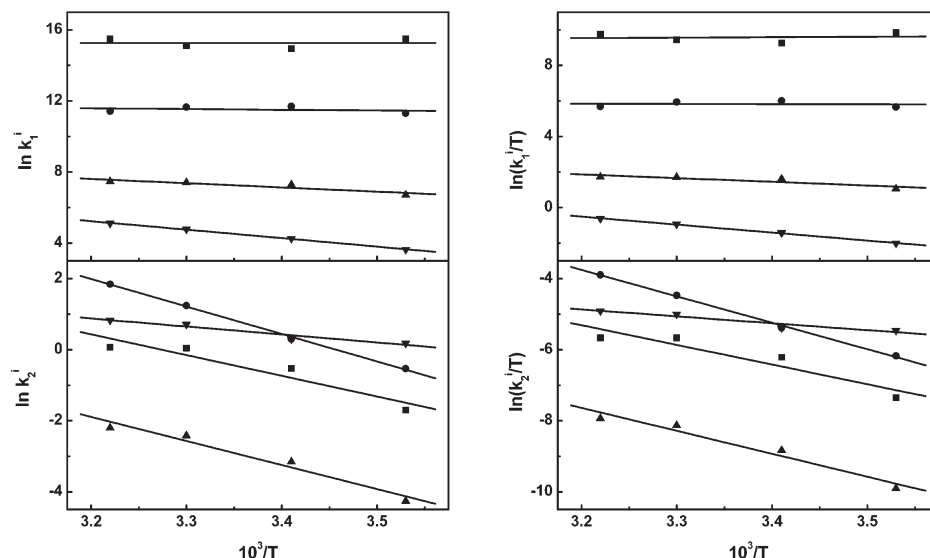
Figure 3. Arrhenius and Eyring plots for the formation ( k_1^i ) and hydrolysis ( k_2^i ) of the Schiff bases of pyridoxal 5'-phosphate and L-tryptophan: (■) i = 0 ; (●) i = 1 ; (▲) i = 2 ; (▼) i = 3
