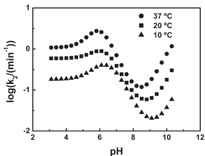
Figure 2. Plot of \log k_2 vs. pH for the Schiff bases of pyridoxal 5'-phosphate and L-tryptophan at different temperatures. Points calculated using Eqn (3) and data from Table 2
