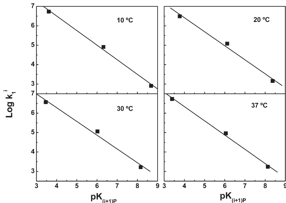
Figure 1. Brønsted plots for the PLP-TRP system at different temperatures
